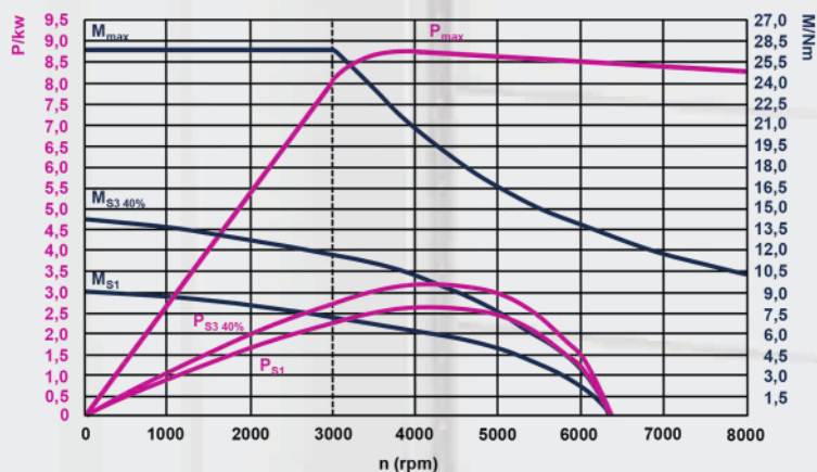
Driven tool 8,000 rpm
