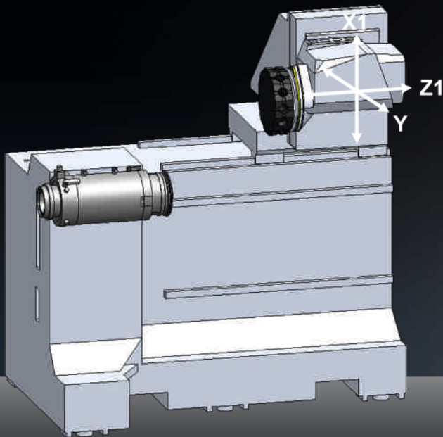
Version without tailstock
