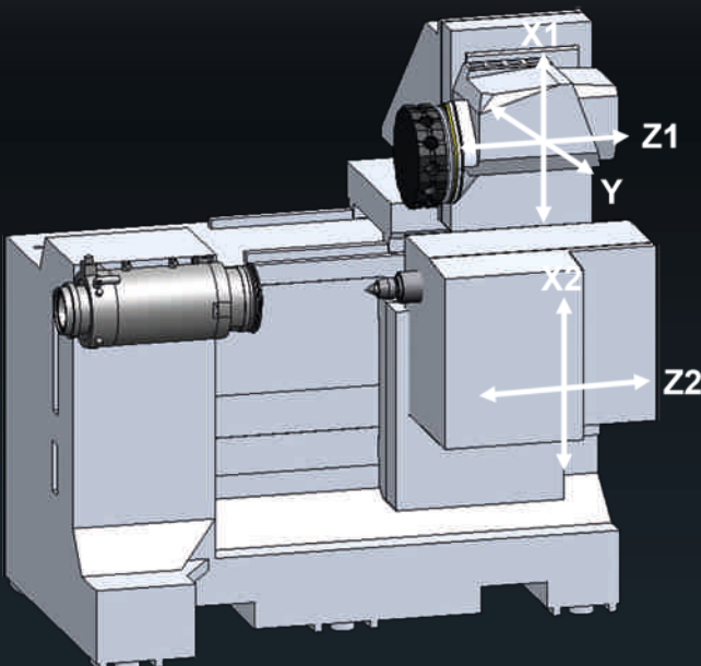
With CNC-tailstock with X2/Z2 axis
