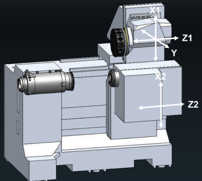
With sub-spindle on positioning slide
